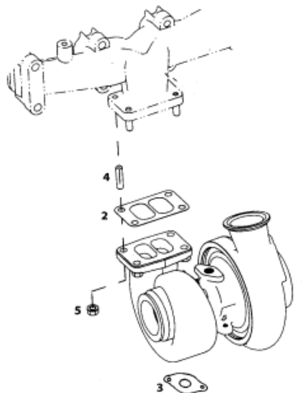
TURBOCHARGER (LOW MOUNT) (EURO II)
