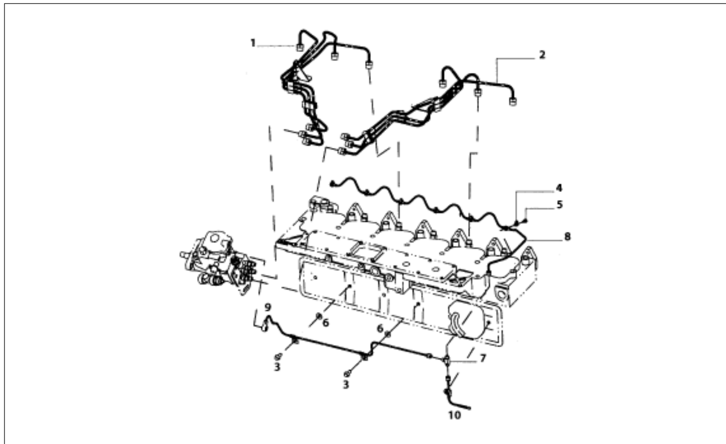
PLUMBING, FUEL (EURO II)
