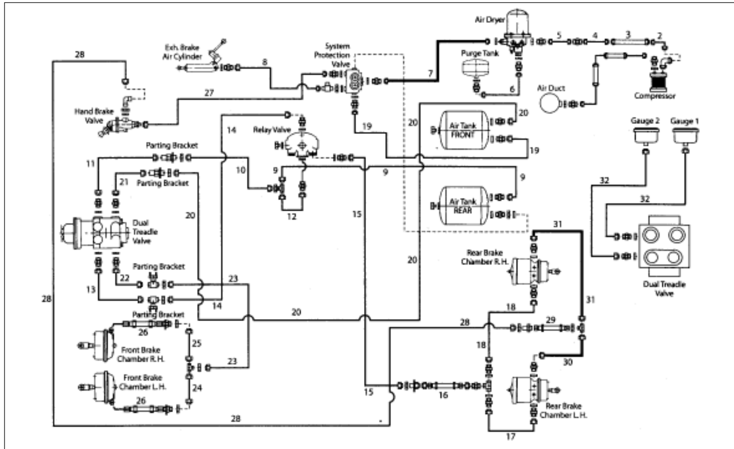
AIR BRAKE LINES WITH RELAY (NEW)
