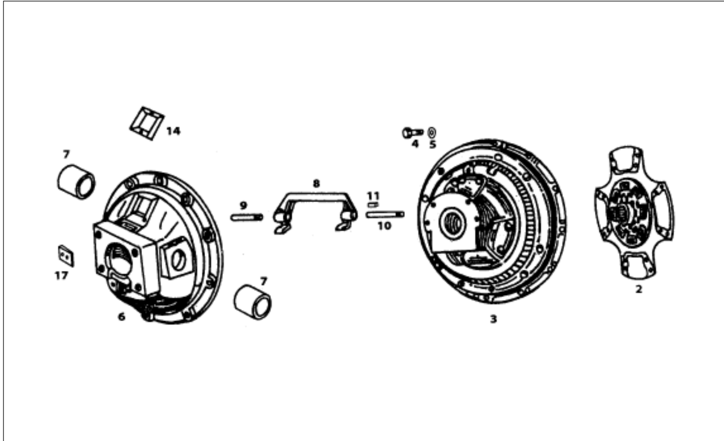
CLUTCH (352 MM DIA.) COIL TYPE
